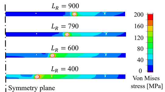
Figure 14 PV module frame stress results for load case 1 (1 kPa uniform pressure).
