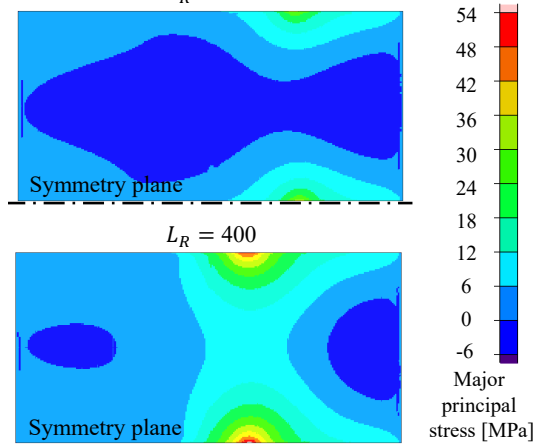
Figure 17 PV module glass stress results for load case 2 (0 to 2 kPa distributed pressure).
