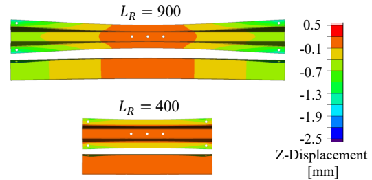
Figure 7 Rail displacement results for load case 1 (1 kPa uniform pressure).
